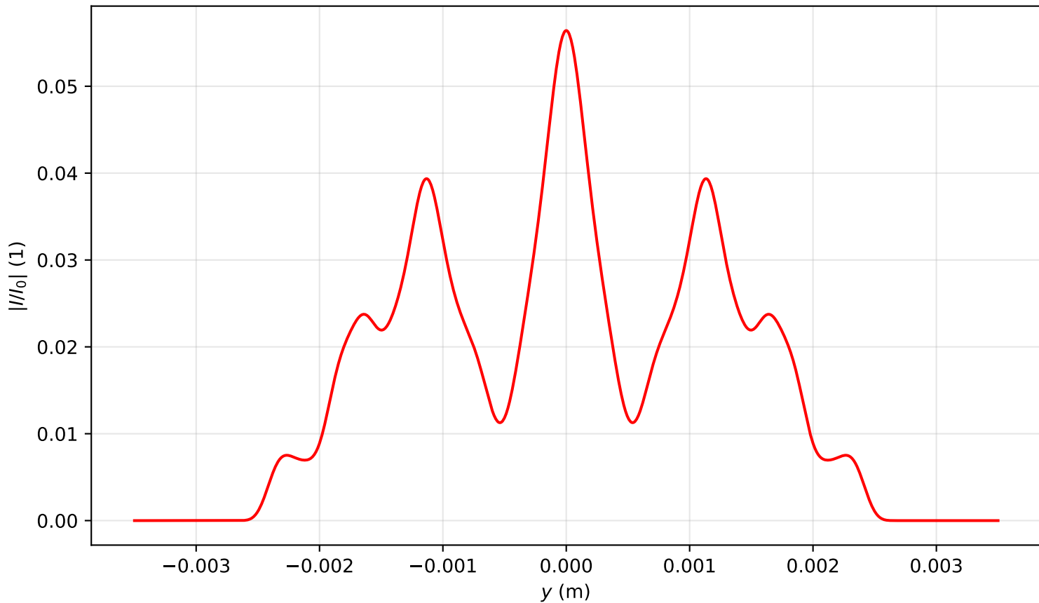
Intensity profile I(x=0, y, z=3.821)/I_0 , P_{in}=8.5P_{cr} , artificial time
